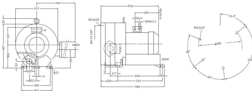
Installation Drawing
