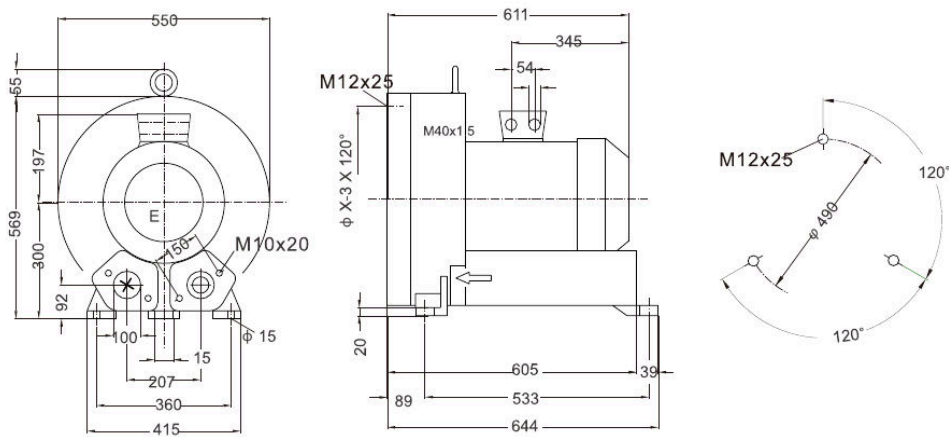
Installation Drawing
