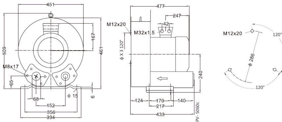
Installation Drawing
