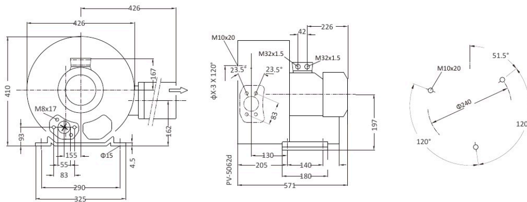
Installation Drawing
