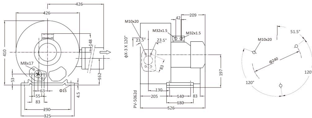
Installation Drawing
