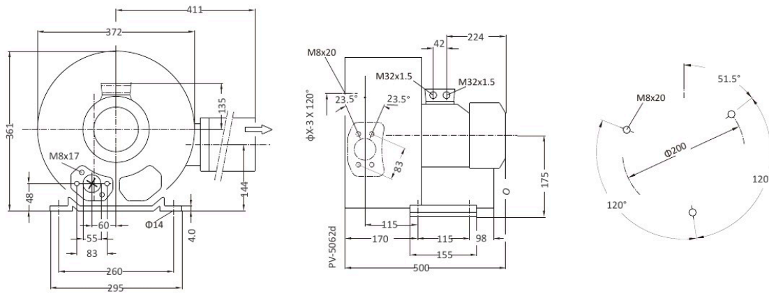
Installation Drawing
