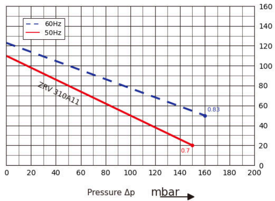
Pressure Performance Curve
