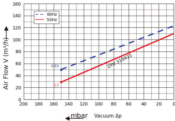
Vacuum Performance Curve
