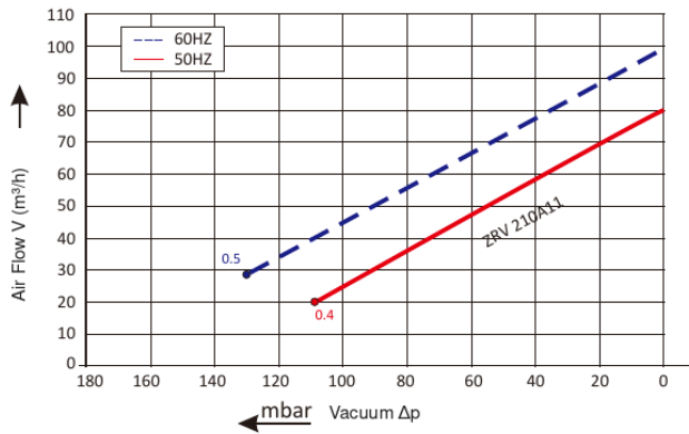
Vacuum Performance Curve
