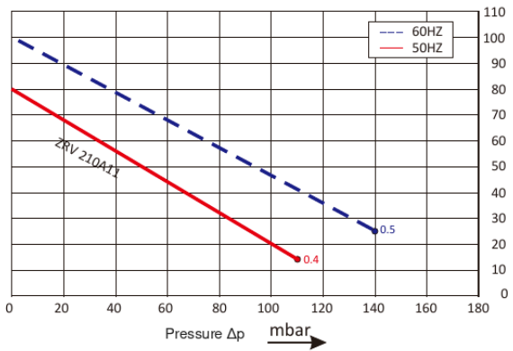
Pressure Performance Curve
